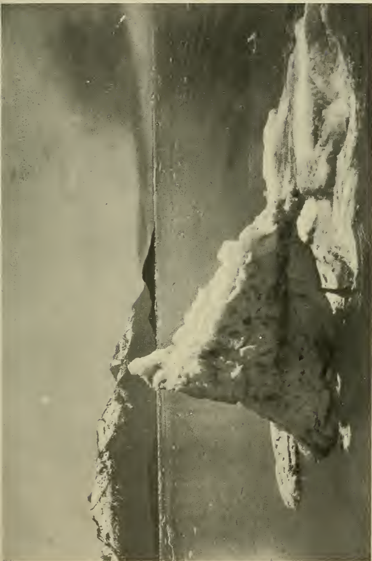
ICE FLOE, ANTARCTIC.
